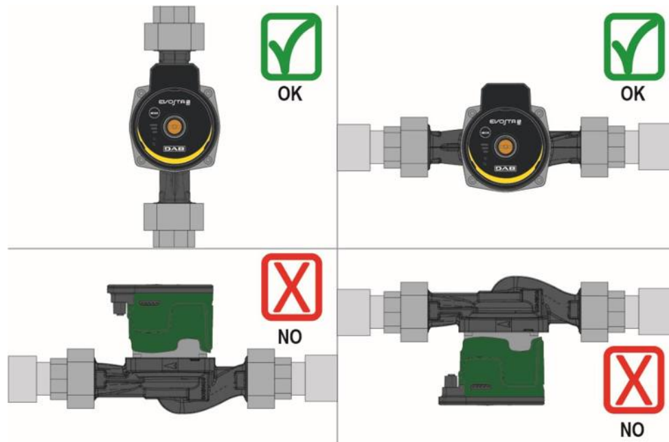
Figure 13: Assembly position
