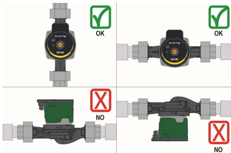
Abb. 13: Montageposition
